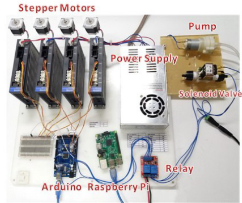
Figure 2. Control system hardware for FarmBot
