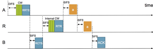
Figure 1. Message handshaking of 2-PSP
