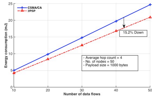
Figure 2. Energy consumption of 2-PSP
