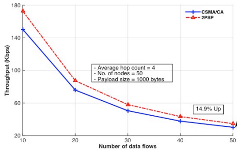
Figure 3. Throughput as a function of flow increase
