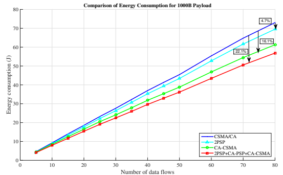
Figure 3. Comparison of energy consumption for CSMA/CA, 2PSP, CA-CSMA, and CA-2PSP
