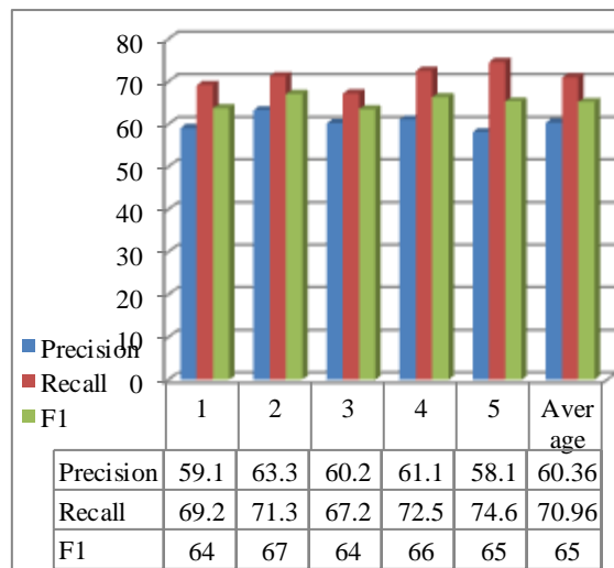
Figure5. Cross Validation Result
