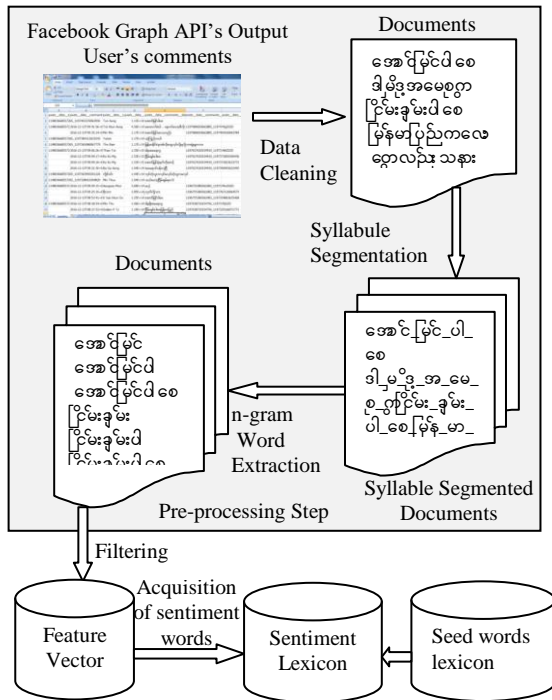
Figure3. Sentiment Lexicon Construction
